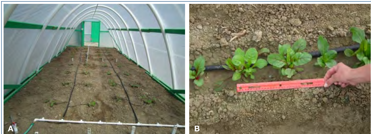
Figure 6.1. Drip irrigation in high tunnels at the University of Wyoming Research and Extension Center in Powell; a) spaghetti tubes and b) in-line emitter drip tubing.
