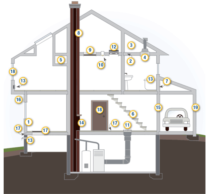
Air Sealing Trouble Spots
