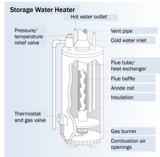
"Natural gas storage water heater" by US Department of Energy http://energy.gov/eere/energybasics/articles/conventional-storage-water-heater-basics
